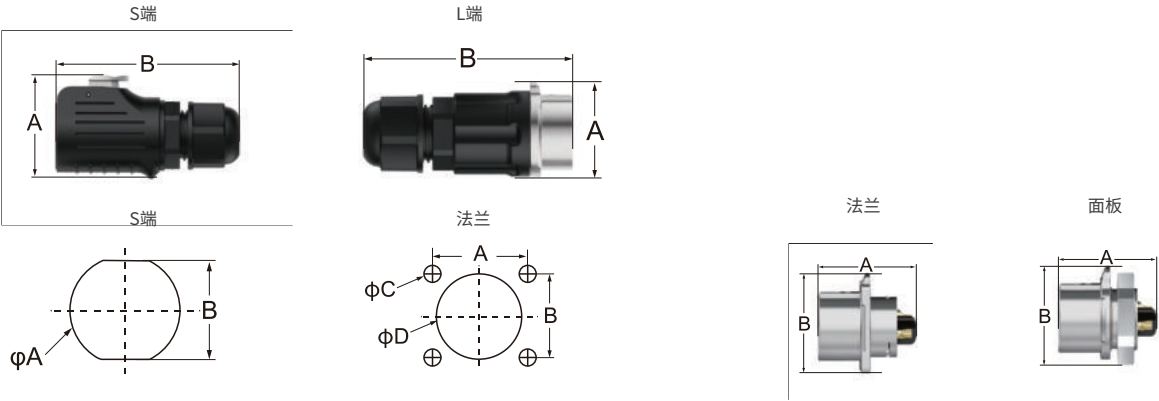
连接器机械尺寸 Mechanical dimensions of the connector
