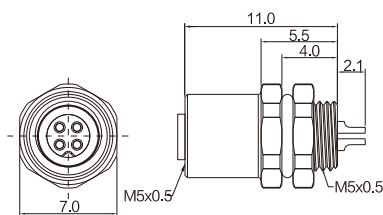
M5母头/Female molded cable
