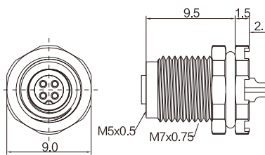
M5母头/Female molded cable
